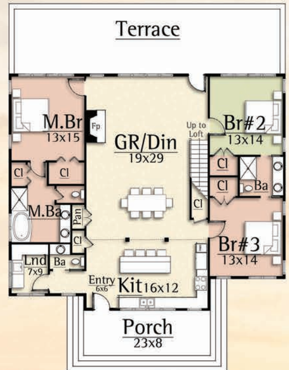
Main Level 2,012 square feet
